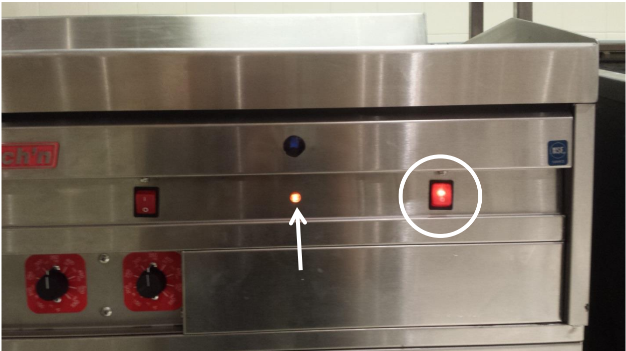
Figure 2: To validate that the unit is operational, turn on one set of burners by pushing the button (circled above). Pilot should light and indicator light should illuminate (indicated by the arrow).
