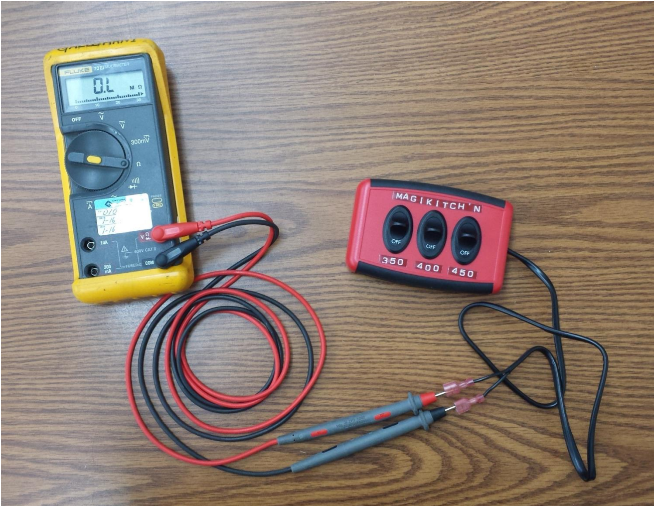
Figure 15: To verify the calibration device, connect your multi meter/ohm reader as shown above.
