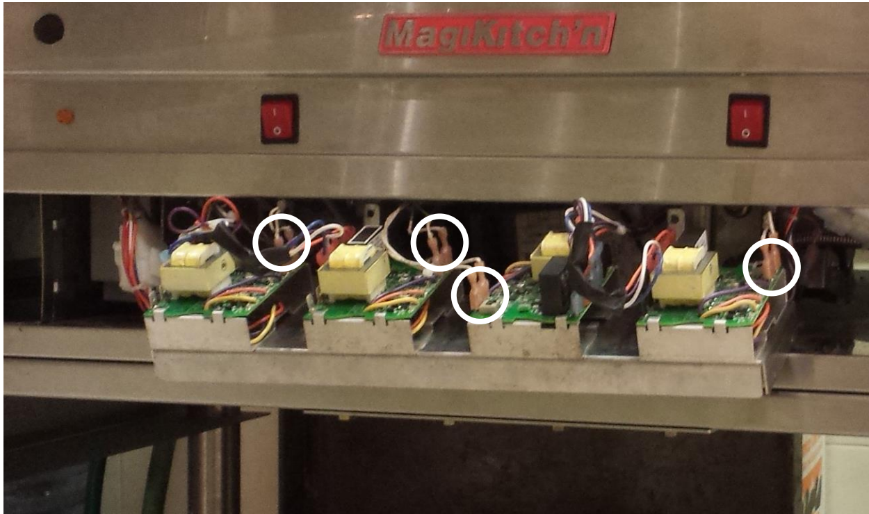
Figure 14: Repeat all of the above steps for each of the Solid State Thermostat controls. Making sure to re-install the units Thermostat plugs when complete with each controller (Thermostat wires do not have to be in any particular order/position).
